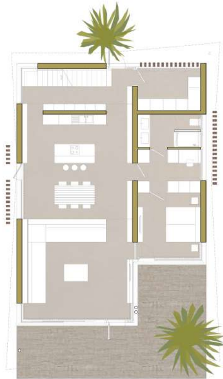
GROUND FLOOR / PLANTA BAJA
