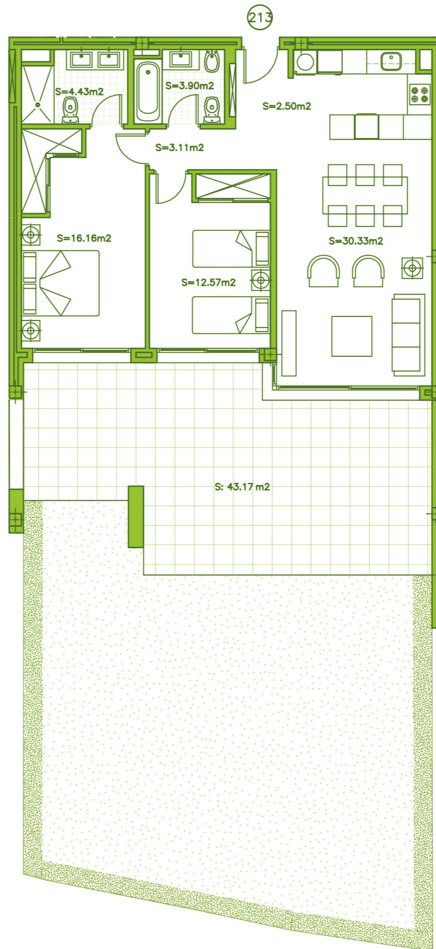
Ground floor
