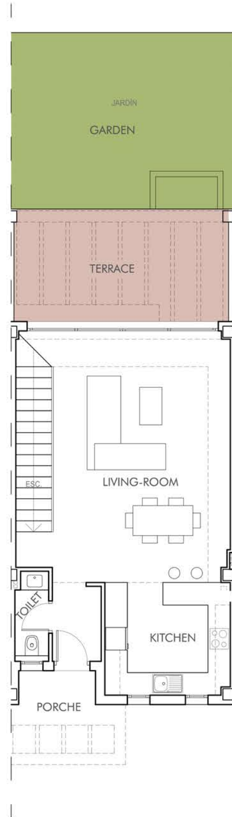
GROUND FLOOR
